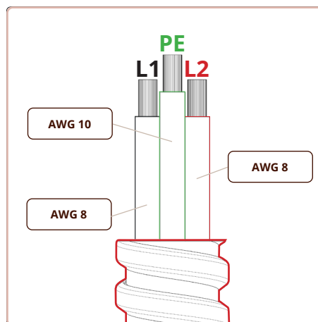
Wiring diagram 208 - 240 V ~ Max. 11.520 Watt
