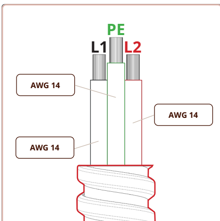
Wiring diagram 208 - 240 V ~ Max. 3.840 Watt
