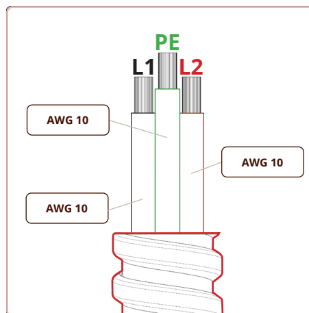
Wiring diagram 208 - 240 V ~ Max. 6.840 Watt
