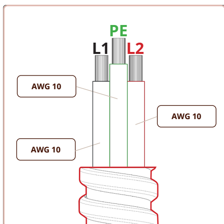
Wiring diagram 208 - 240 V ~ Max. 6.000 Watt
