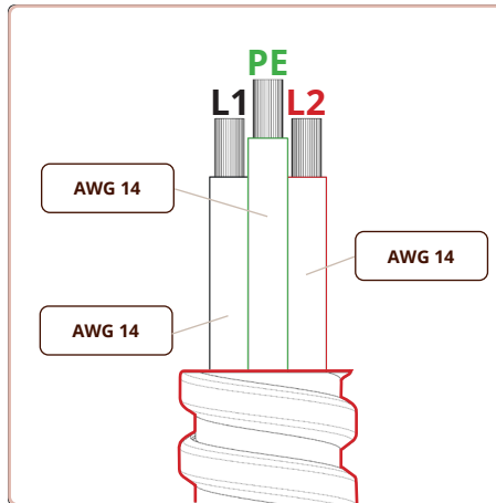
Wiring diagram 208 - 240 V ~ Max. 2.100 Watt
