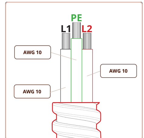
Wiring diagram 208 - 240 V ~ Max. 7.680 Watt
