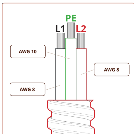
Wiring diagram 208 - 240 V ~ Max. 10.680 Watt
