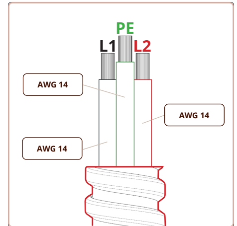
Wiring diagram 208 - 240 V ~ Max. 3.000 Watt
